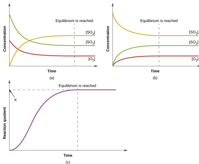
Figure 17.3a: (a) The change in the concentrations of reactants and products is depicted as the 2 \text{SO}_2(g) + \text{O}_2(g) \rightleftharpoons 2 \text{SO}_3(g) reaction approaches equilibrium. (b) The change in concentrations of reactants and products is depicted as the reaction 2 \text{SO}_3(g) \rightleftharpoons 2 \text{SO}_2(g) + \text{O}_2(g) approaches equilibrium. (c) The graph shows the change in the value of the reaction quotient as the reaction approaches equilibrium (credit: Chemistry (OpenStax), CC BY 4.0).
